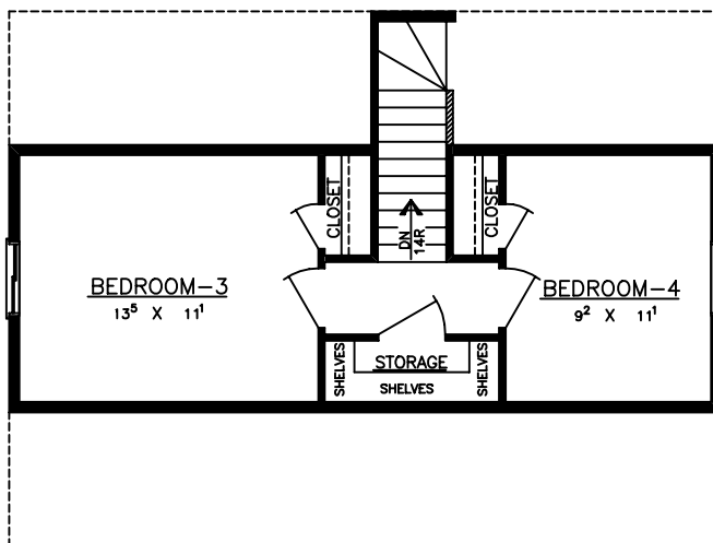
SECOND FLOOR AREA = 384 S.F.
