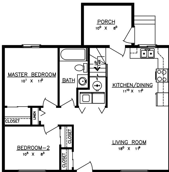
MAIN FLOOR AREA = 768 S.F.
